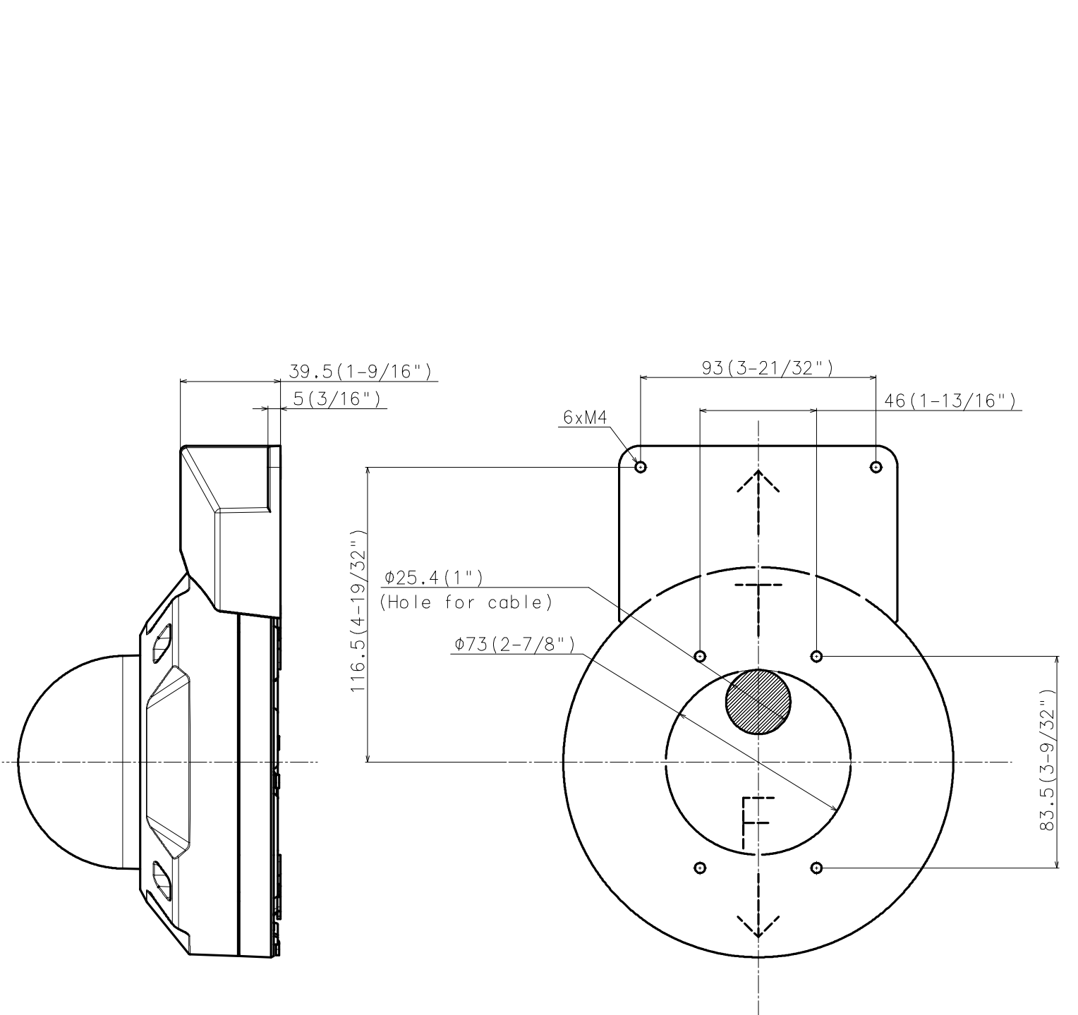
Template for mounting
