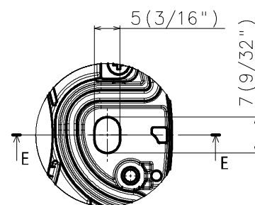
Detail D (2:1) Symmetrical
