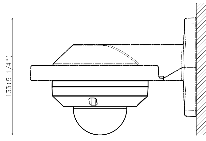
Attach to WV-QWL500-W
