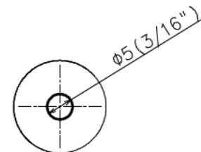
Detail Z (2:1) Hole size (Position D, E, G)
