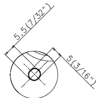
Detail Y (2:1) Hole size (Position A, C, F)
